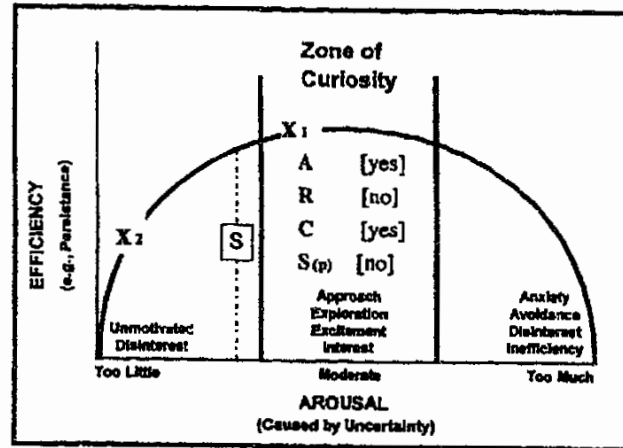
Figure 5: A, C, but no R and hence no S(p)
