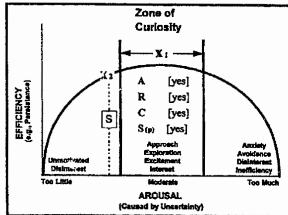
Figure 7: A, R, C, S_{int} are all present
