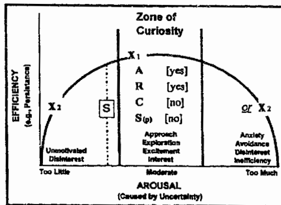
Figure 6: A, R, but no C, S (p)
